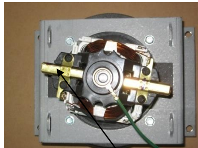
"Quick Change" Brush Motor Quick Change Brush
