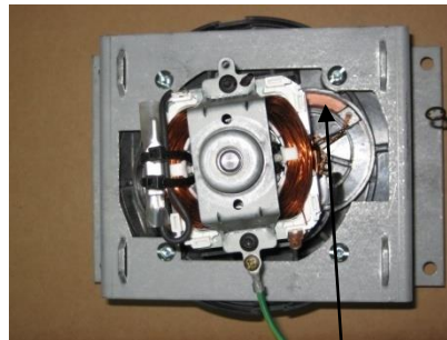
"Infinity" Brush Motor Infinity Curved Motor Brush
